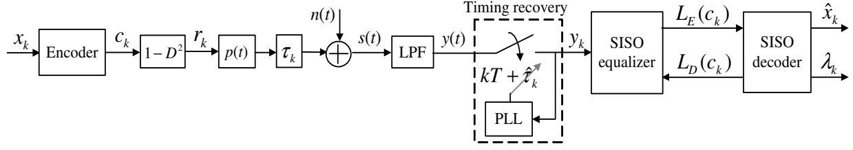
Fig. 1. A channel model with a conventional receiver.
