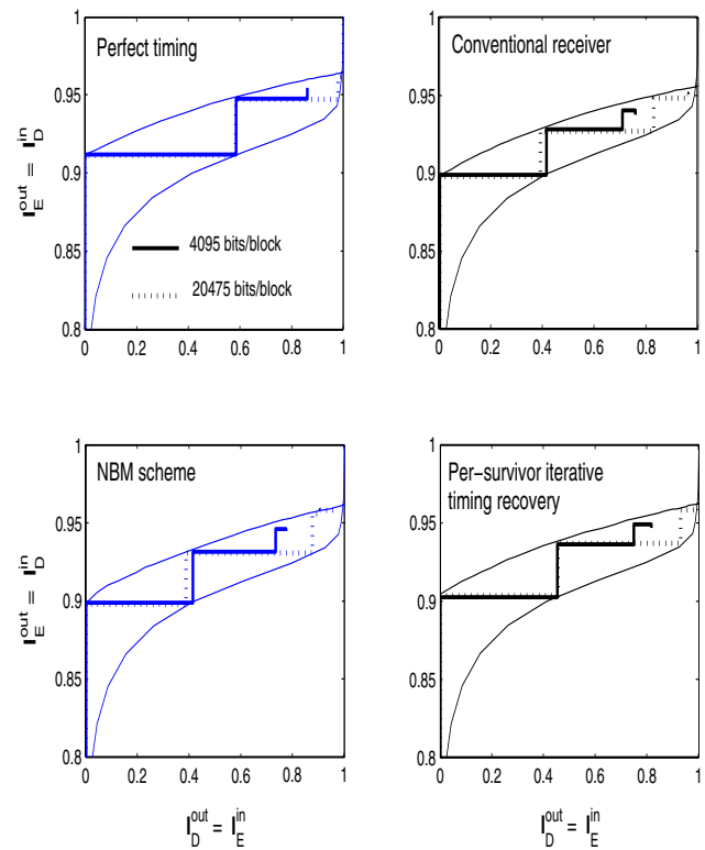
Fig. 6. System trajectories at E_b/N_0 = 5 dB and \sigma_w/T = 0.5\% . The solid lines are based on the coded block length of 4095 bits, whereas the dashed lines are based on the coded block length of 20475 bits
