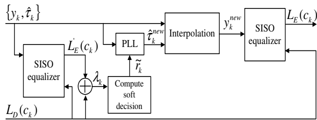
Fig. 3. Simulation setup for generating the equalizer transfer characteristic of the NBM scheme.
